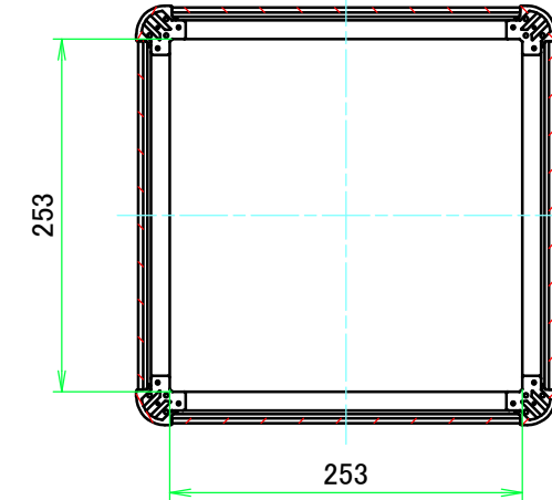
C-C (1:6)
